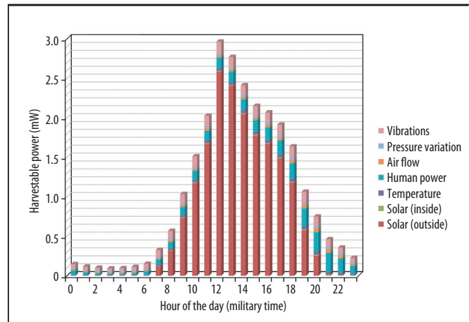
Figure 5. Results of correlating seven energy-harvesting sources with each source’s availability over an average work-day. Each segment represents the average amount of power that an individual could expect to harvest at any given time when all sources are being deployed. Nightly blackouts are a particular challenge and will require efficient energy storage mechanisms.
