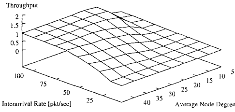
Figure 4: Throughput produced by allocation protocol.
