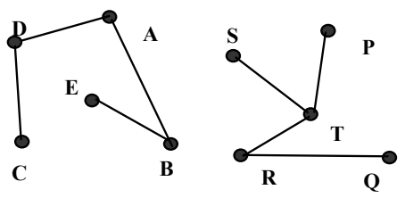
G(A,B,C,D,E,P,Q,R,S,T) is a forest G(A,B,C,D,E) is a tree
