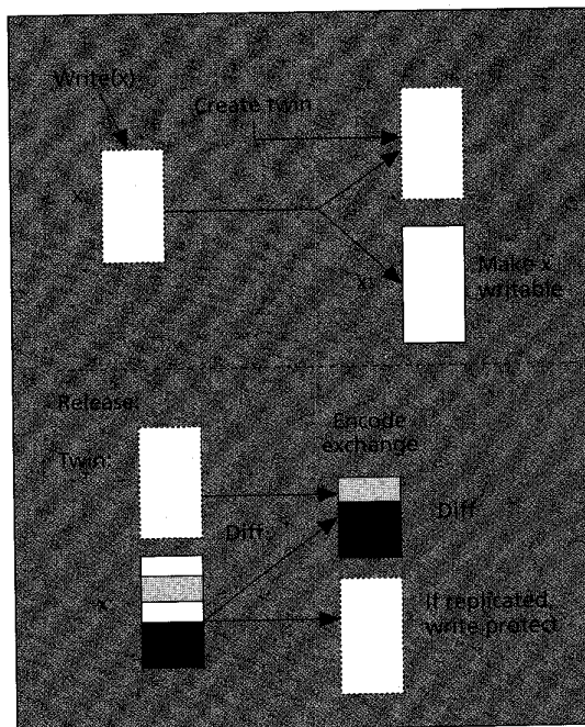
Figure 7. Diff creation.
